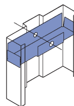
Snap-in Prepared Opening Anchor
