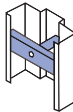
Twist in Prepared Opening Anchor
